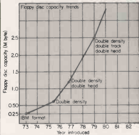
Figure 3. Projection of storage capacity against technique. single and double information bit densities also remains about the same.
